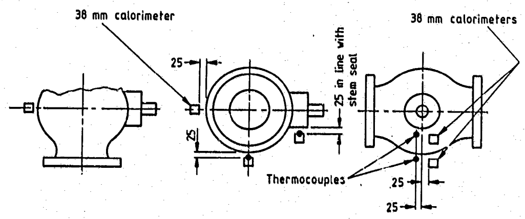
Figure 4. Location of calorimeter cubes and flame environment thermocouples for valves larger than DN 150 (NPS 6) (see A.5.1)
