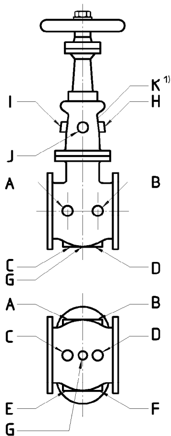
Figure 3 — Location of tapings for auxiliary connections
