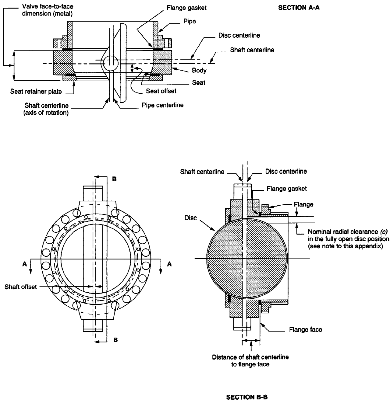
Figure A-2—Nomenclature and Explanation of Offset-Seat-Type Construction (Category B)
